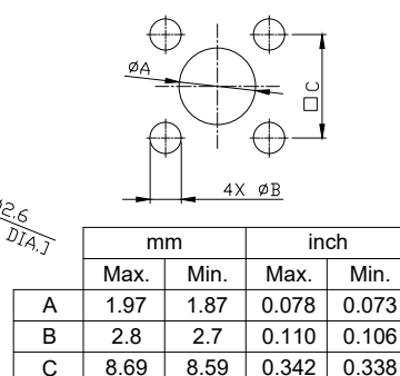
Mounting Dimensions
